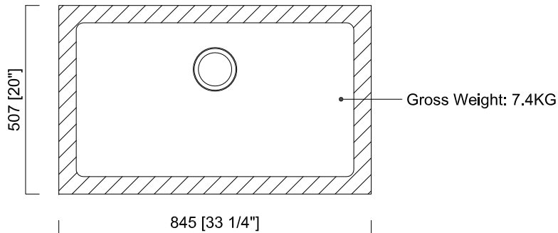
PACKAGING DIAGRAM
