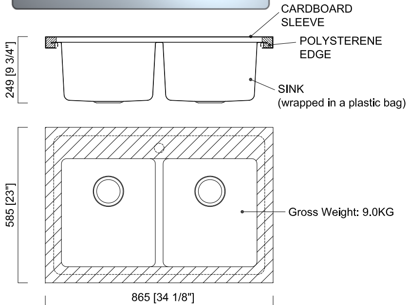
PACKAGING DIAGRAM
