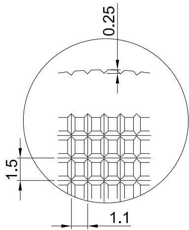
KNURLED DETAIL 20:1
