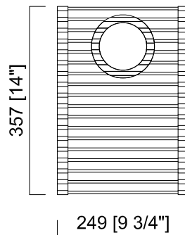
Rolla-Grid (CN3625RG) 1pcs
