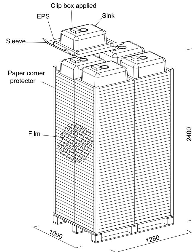
PACKAGE DIAGRAM (Waste Kit & Drain Pipe packed on separate pallet)
