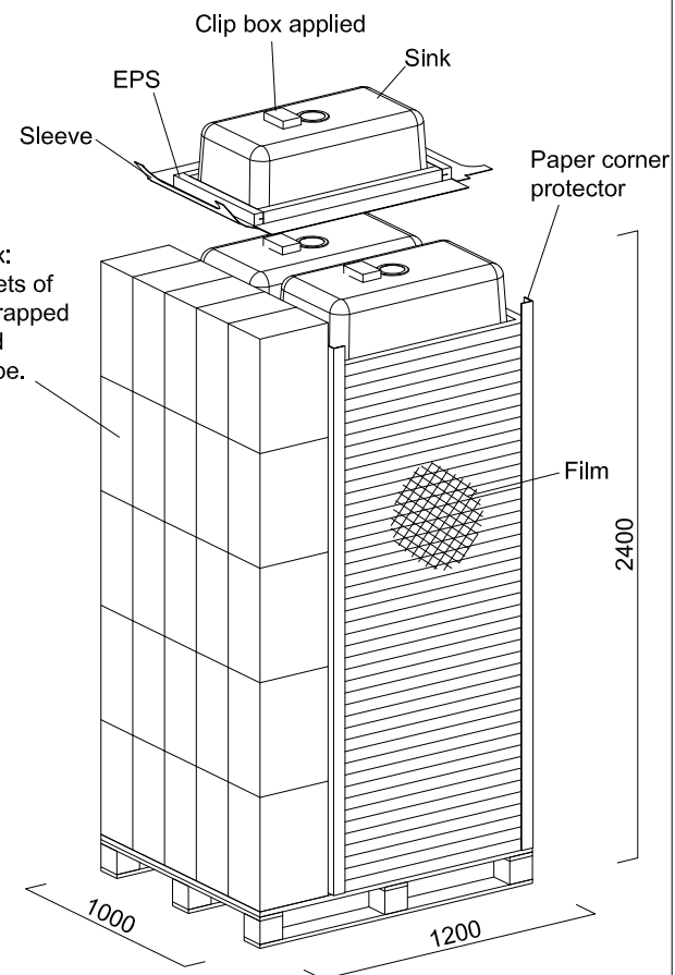
PACKAGE DIAGRAM
