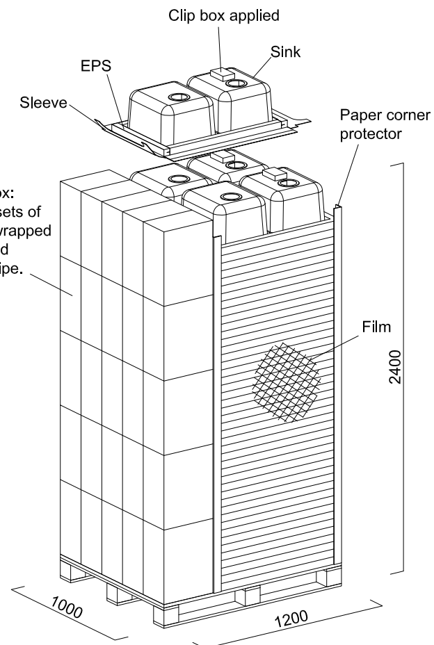
PACKAGE DIAGRAM
