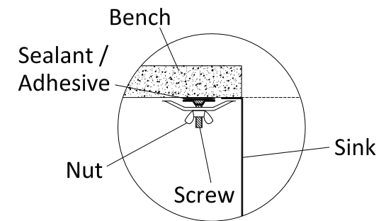
Undermount clips instruction (UMG)
