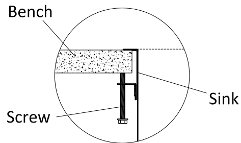
Inset clips instruction (ICM)
